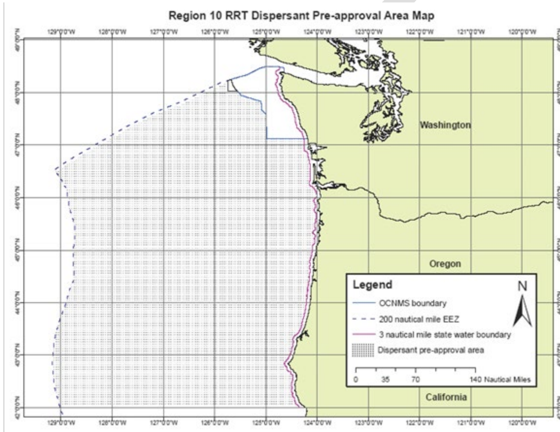
Figure 7110-1 Dispersant Pre-Authorization Zone
