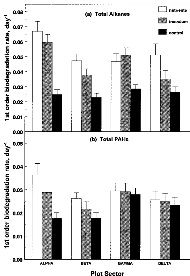
FIGURE 7. First-order biodegradation rates of (a) total target alkanes and (b) total target aromatics according to location within the intertidal zone ( \alpha -sector is closest to the high dune area; \delta -sector is closest to the water) (error bars represent \pm one standard deviation unit).
