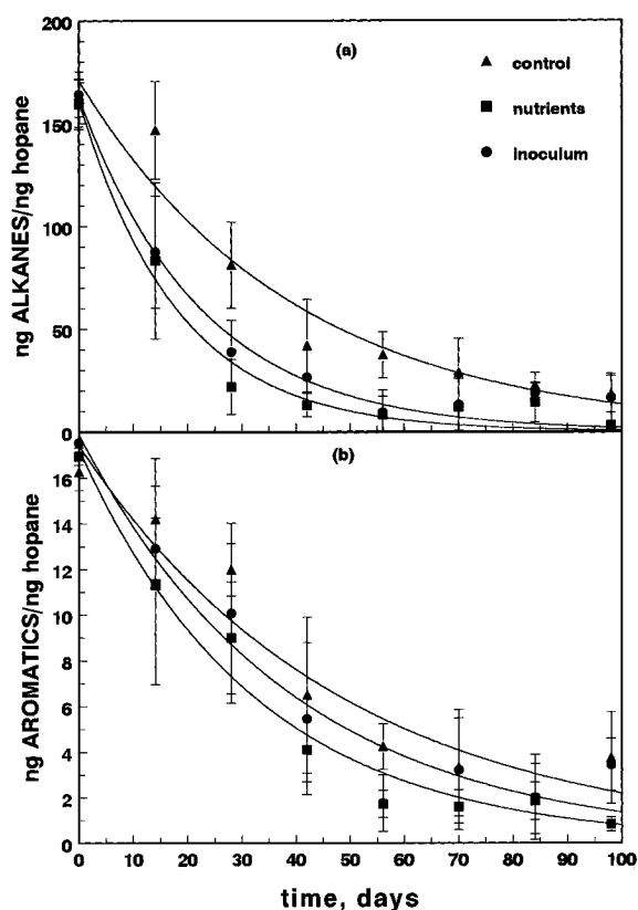
FIGURE 4. First-order declines in (a) total target alkanes ( nC_{10} – nC_{35} plus pristane and phytane) and (b) total target aromatics, including alky-substituted homologues (error bars represent \pm one standard deviation unit).
