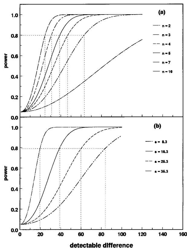
FIGURE 8. Statistical power curves for hopane-normalized total alkanes (a) for varying n and constant \sigma of 16.3 and (b) for varying \sigma and constant n of 5.
