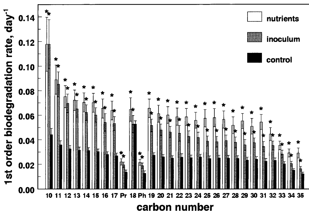
FIGURE 5. First-order biodegradation rates of all individual normal and branched alkanes computed by nonlinear regression of the data over the entire 14-week experimental time period [error bars represent \pm one standard deviation unit, and asterisks identify significant differences from untreated control plots ( p < 0.05 )].
